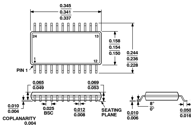
COMPLIANT TO JEDEC STANDARDS MO-137AE Figure 67. 24-Lead Shrink Small Outline Package [QSOP] (RQ-24) Dimensions shown in inches
